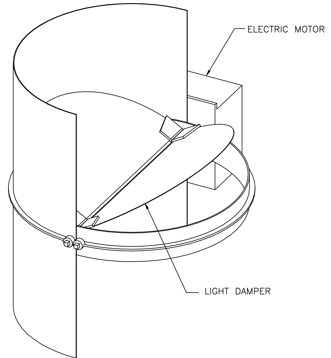
3D CUTAWAY VIEW - DETAIL A SCALE N.T.S.
