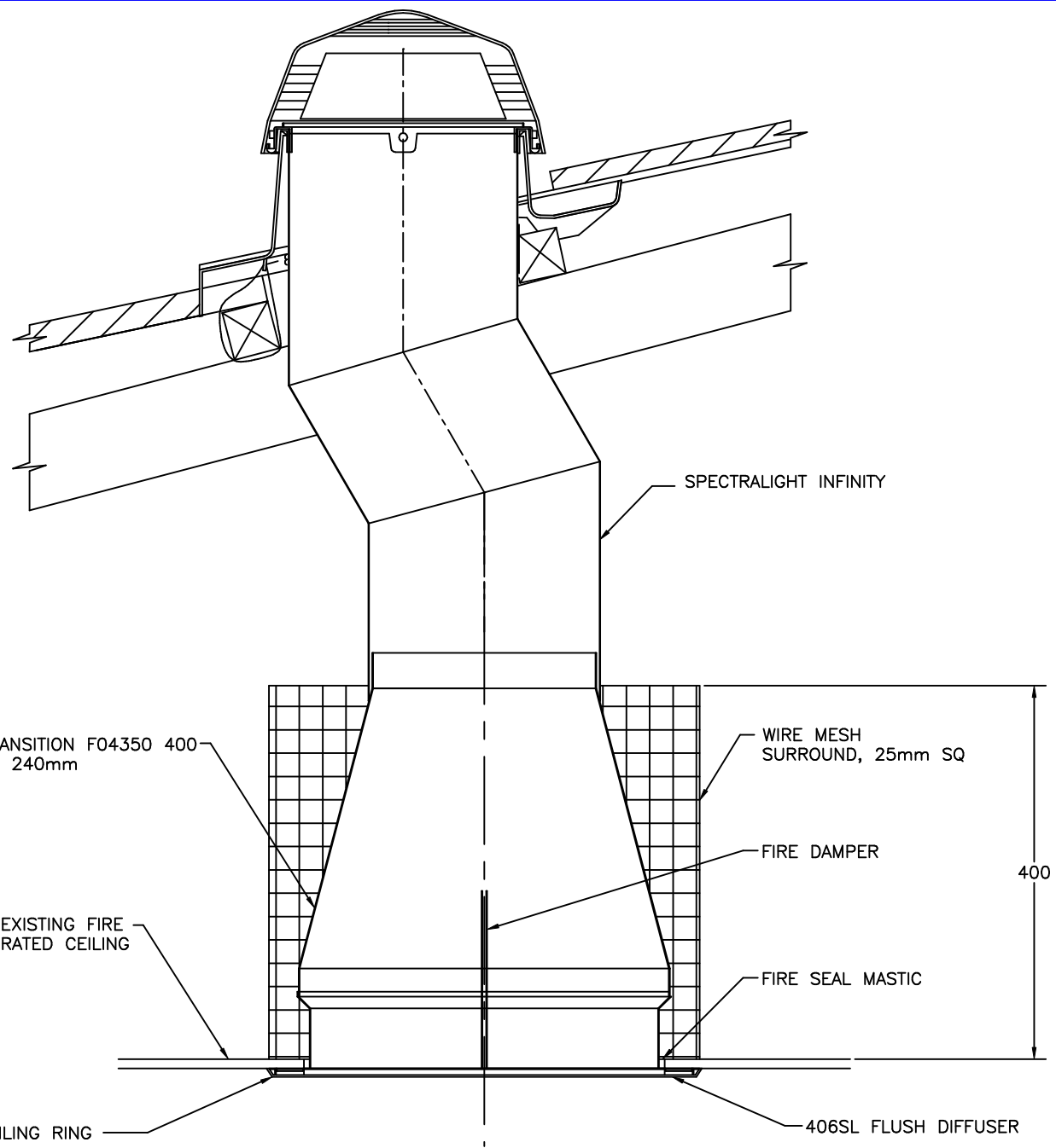
TYPICAL CROSS-SECTION SCALE 1:5
