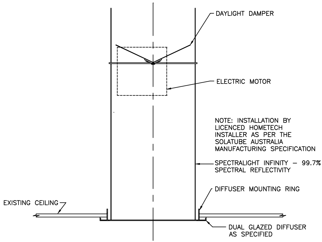
SECTION THROUGH SOLATUBE & DIFFUSER SCALE 1:5
