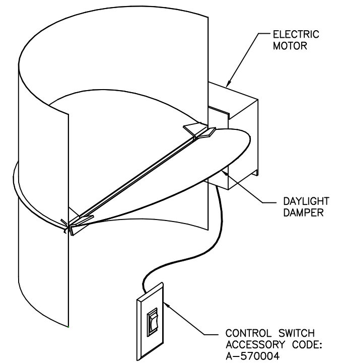
3D CUTAWAY VIEW - DETAIL A SCALE N.T.S.
